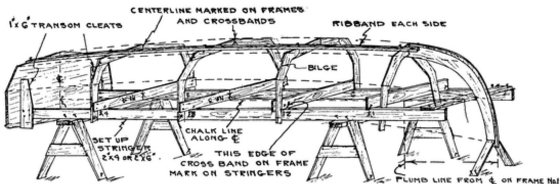
FIG. No. 9 BOAT ERECTED BOTTOM UP—READY TO PLANK.
