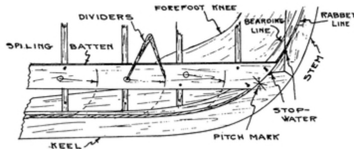
METHOD USED TO LAY OUT A GARBOARD OR A SHUTTER FIG. No.11
