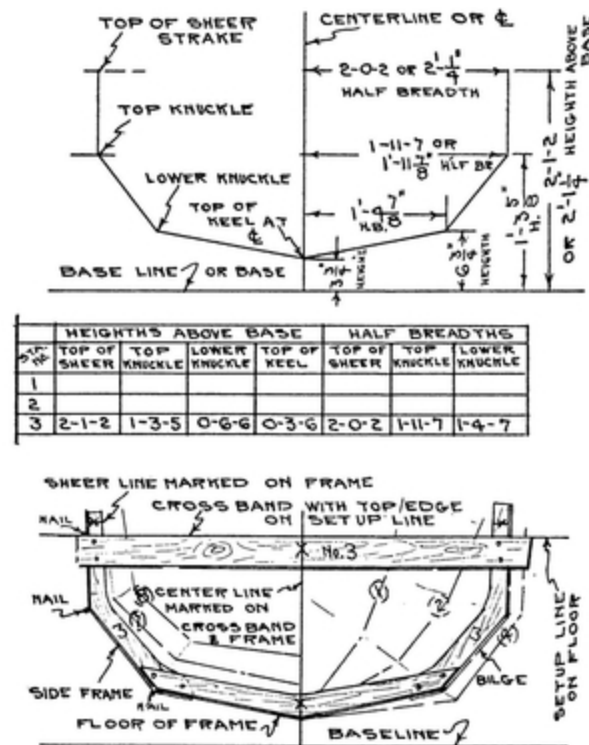
EXPLANATION OF OFFSETS ABOVE, AND BELOW A FRAME OF ONE OF SMALLER BOATS READY TO REMOVE FROM FLOOR FIG. No. 6
