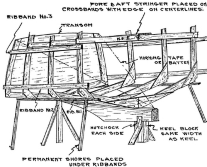
FIG. No. 10 BOAT ERECTED RIGHT SIDE UP.
