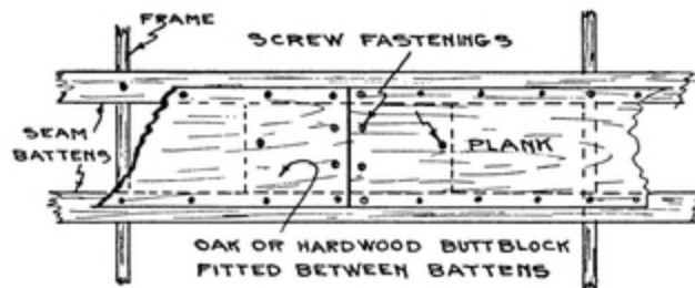
BUTT BLOCK FIG. No. 14.
