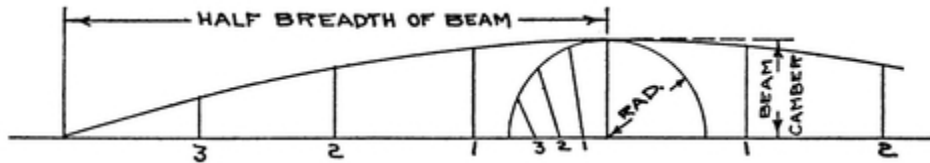
BEAM CAMBER OR CROWN FIG. No. 15
